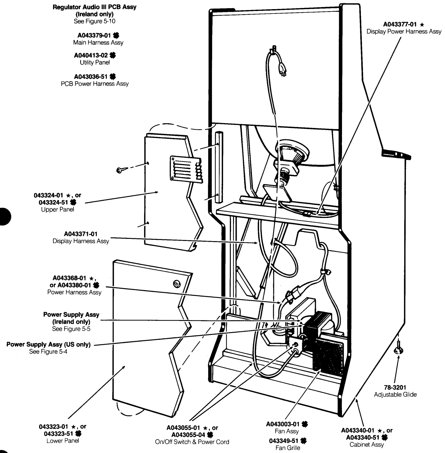
Figure 5-1 Cabinet-Mounted Assemblies, Continued
