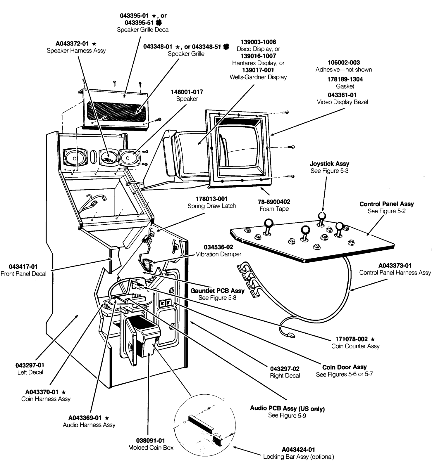
Figure 5-1 Cabinet-Mounted Assemblies A043350-01 and -51 D
