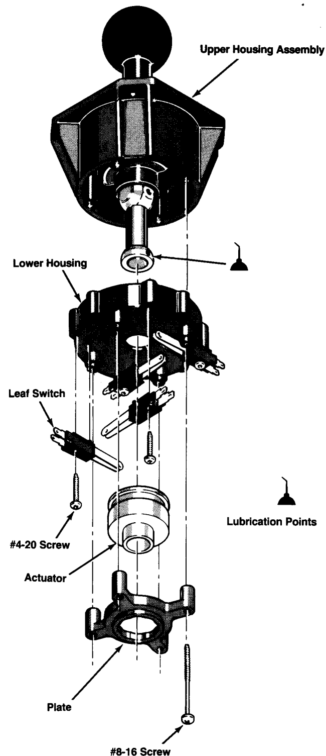
Figure 4-2 Joystick Lubrication
